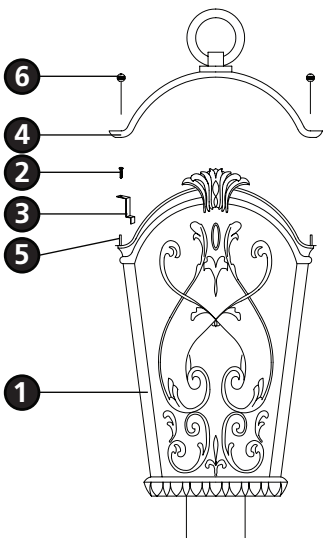
Drawing 2 - Lamp Installation
