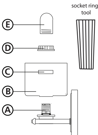
Drawing 3 - Glass Installation
