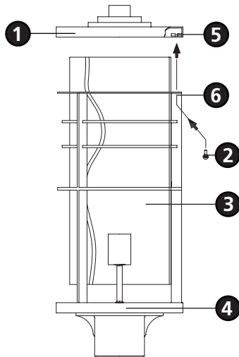
Drawing 2 - Fixture Mounting
